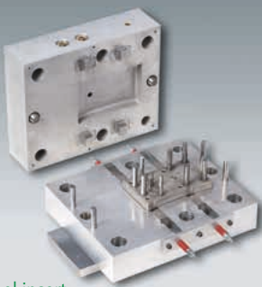
Tool insert
