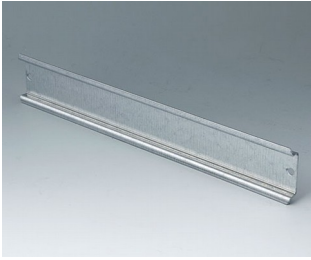
C7117077 Standard DIN rail, Type TH 35 Steel 8.66"x1.38"x0.30"
