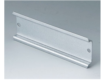
C7112077 Standard DIN rail, Type TH 35 Steel 4.25"x1.38"x0.30"
