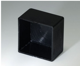
A8022148 POTTING BOXES, Vers. III PA 66 (UL 94 V-2) black RAL 9005 0.88"x0.88"x0.55"
