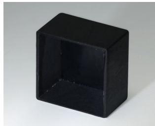
A8020128 POTTING BOXES, Vers. III PA 66 (UL 94 V-2) black RAL 9005 0.82"x0.82"x0.50"
