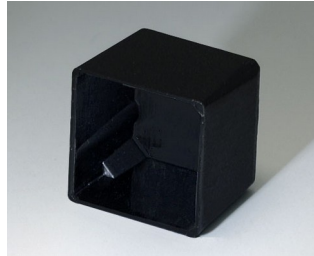
A8014118 POTTING BOXES, Vers. II PA 66 (UL 94 V-2) black RAL 9005 0.55"x0.55"x0.45"
