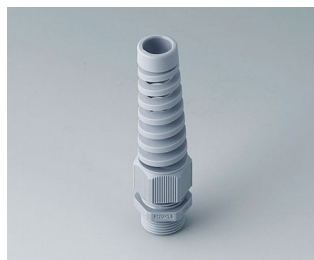
C2320518 Cable gland M20x0.059", bending protection PA silver gray RAL 7001
